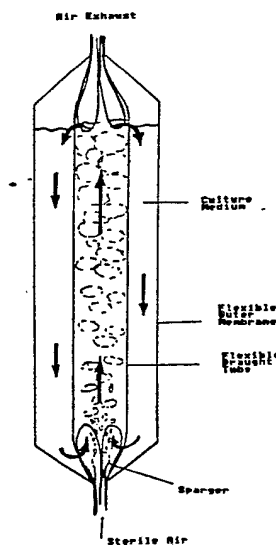
FIGURE 2 AIR LIFT FERMENTER
